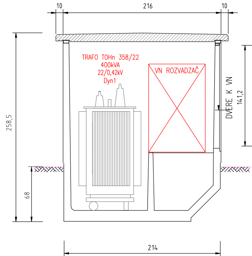
REZ "D-D"
