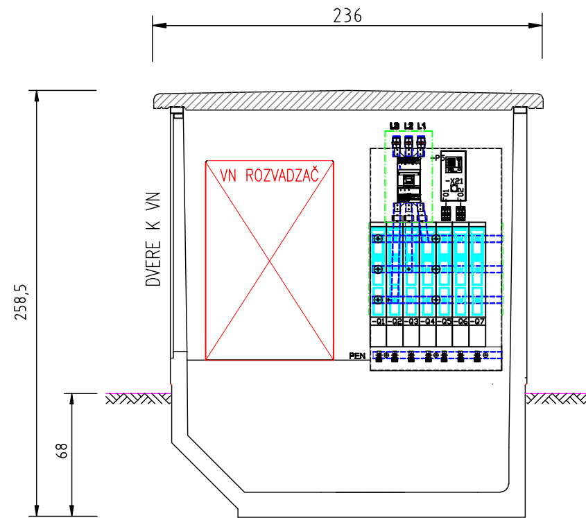
REZ "B-B"
