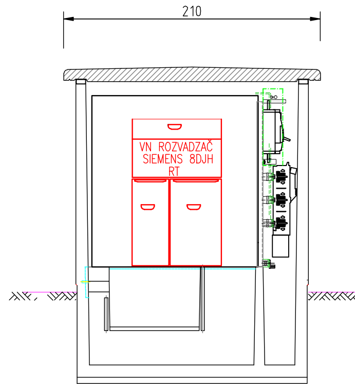
REZ "A-A"
