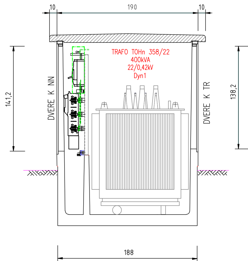
REZ "C-C"
